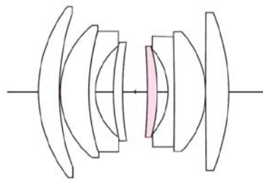
Abnormal partial dispersion lens
